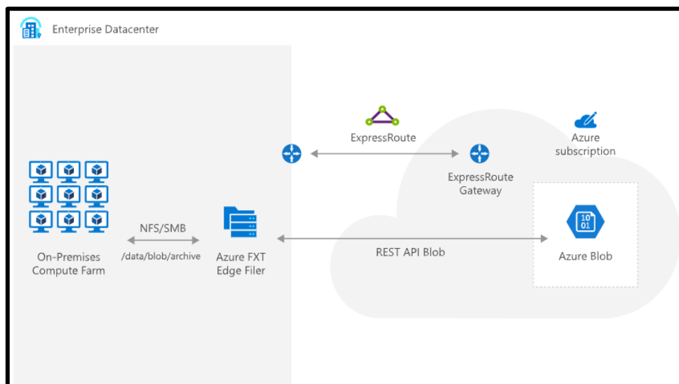
Figure 8 – Aging Data Shift to Azure 11
