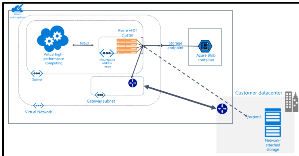
Figure 9 – Avere vFXT for Azure 12
