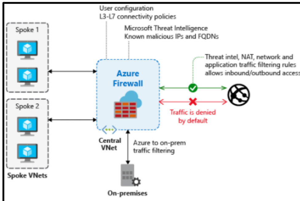
Figure 17 – Azure Firewall 19
