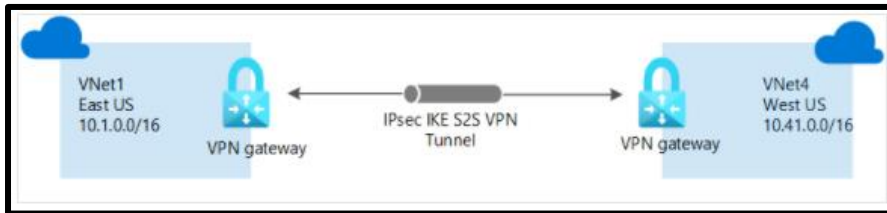
Figure 11 – VNet-to-VNet VPN 14
