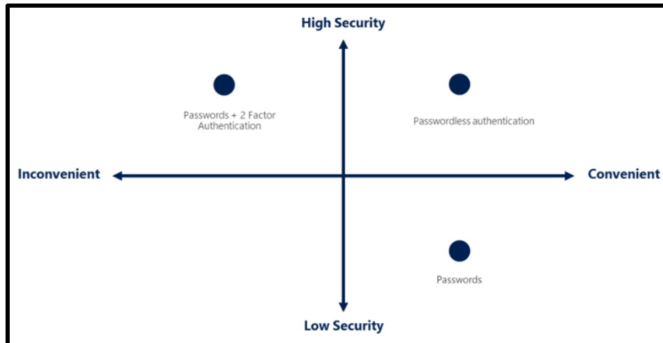
Figure 33 – Passwordless 35
