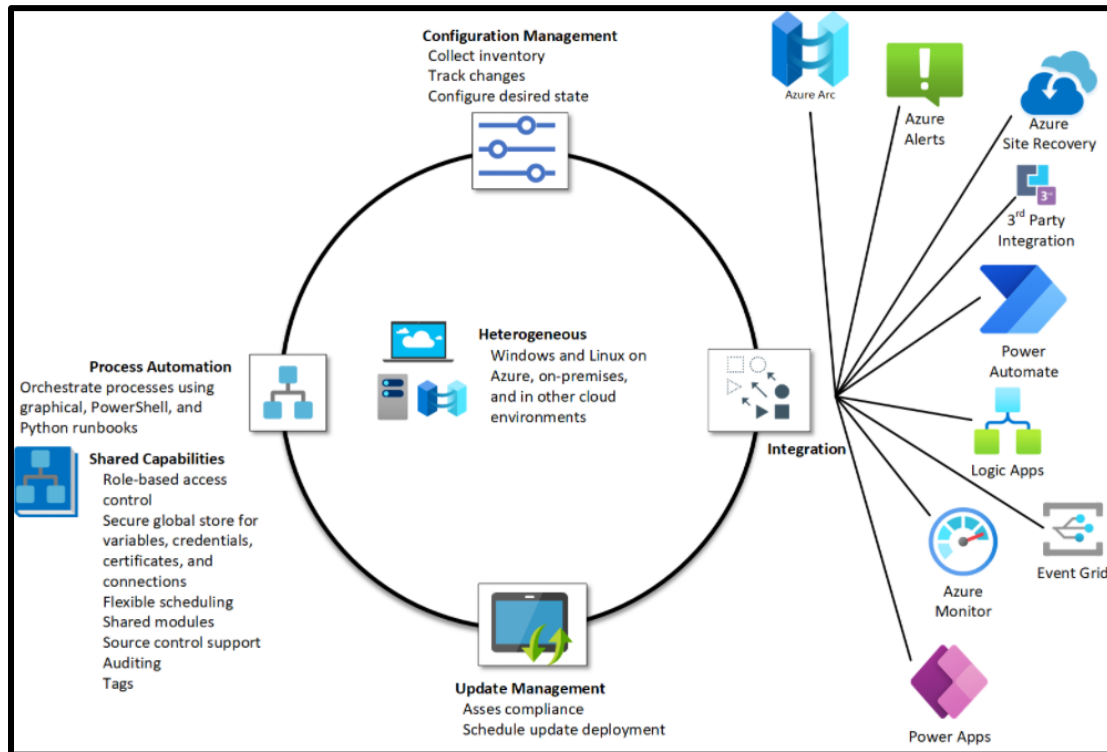
Figure 21 – Azure Automation 24
