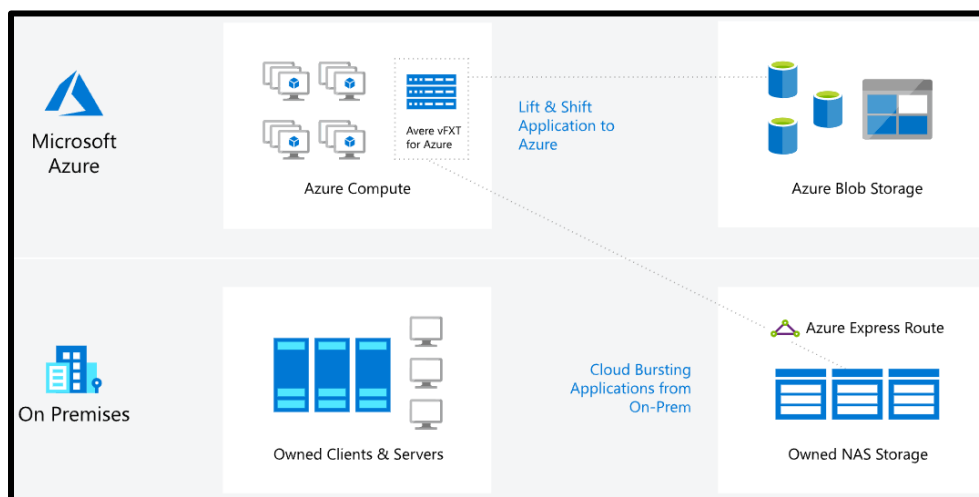
Figure 5 – VFX Rendering Hybrid Deployment using Avere vFXT 8
