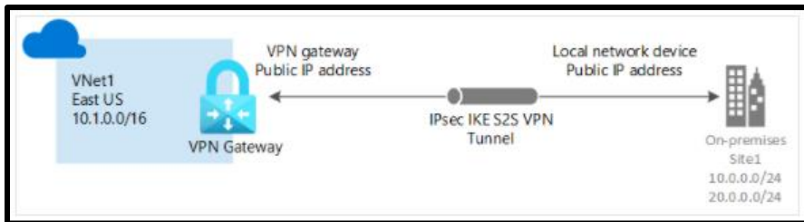
Figure 12 – Site-to-Site VPN 14
