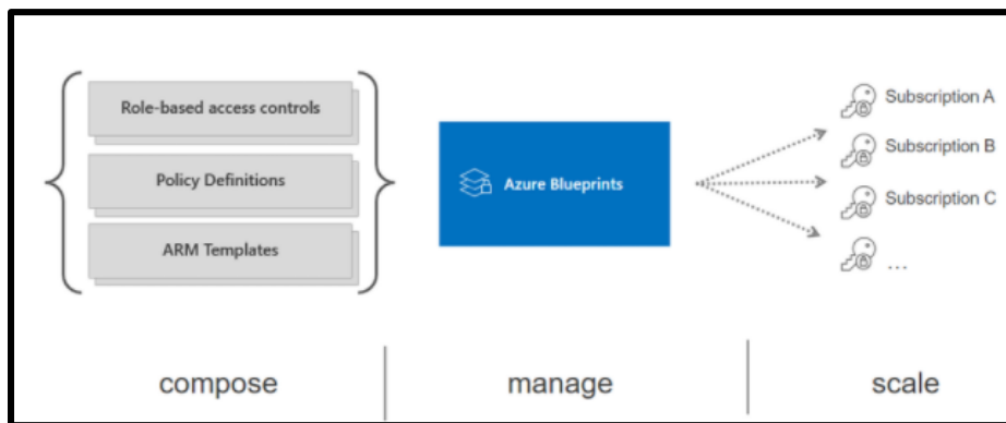
Figure 26 – Azure Blueprints 29
