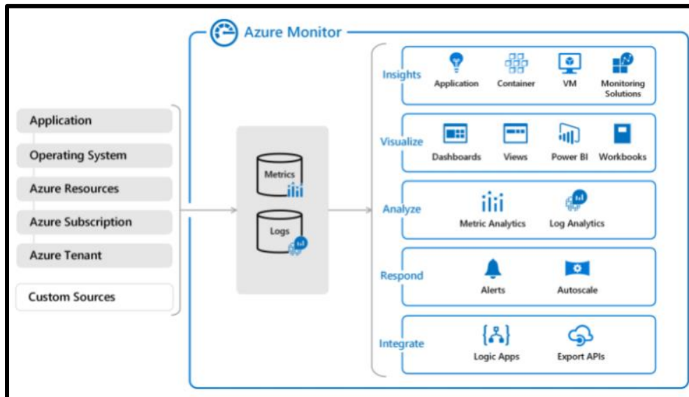
Figure 20 – Azure Monitor 22
