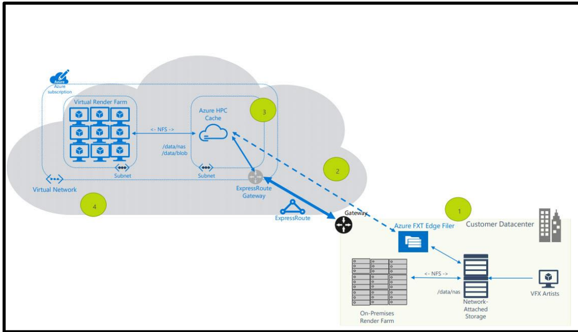
Figure 4 – VFX Rendering Hybrid Deployment using HPC Cache 6
