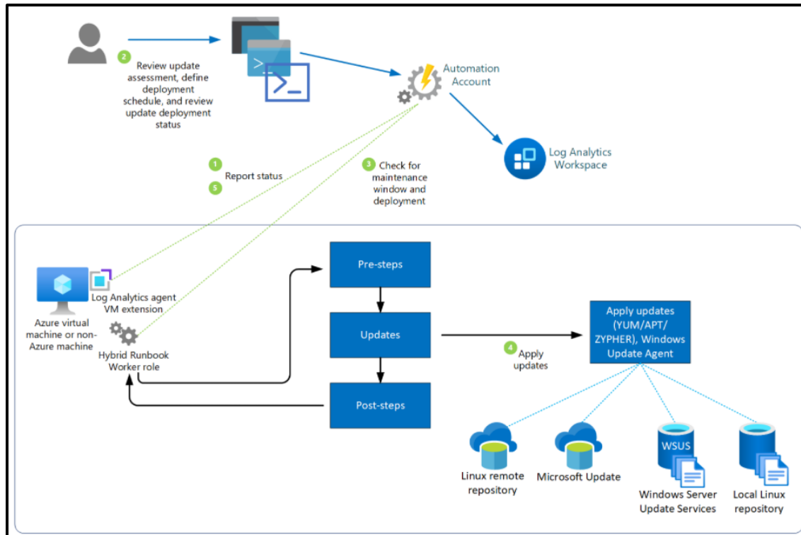
Figure 22 – Update Management 25
