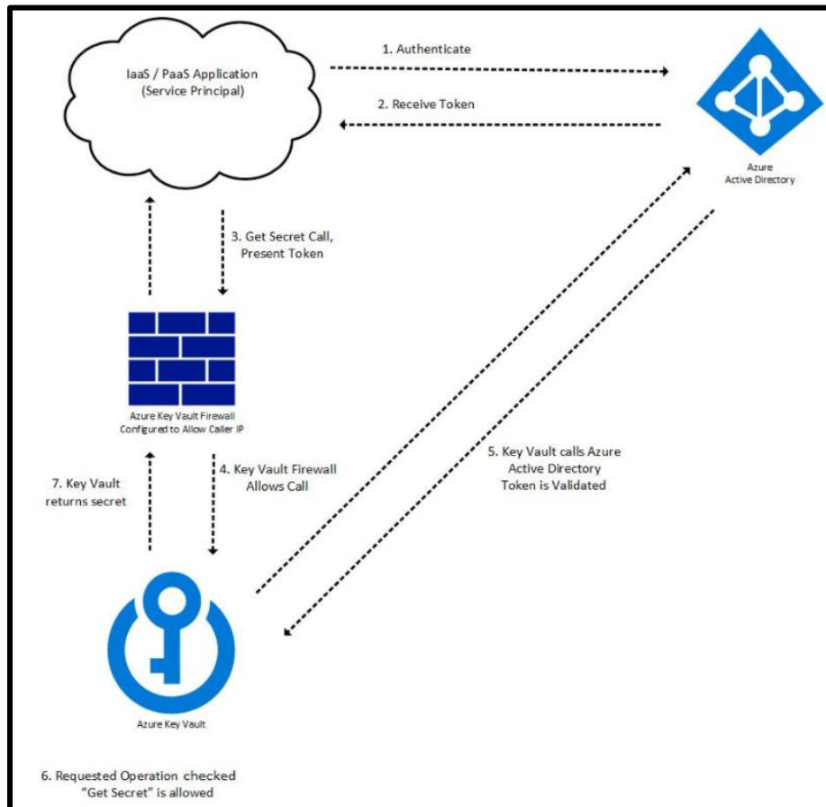
Figure 16 – Key Vault Request Operation Flow 18
