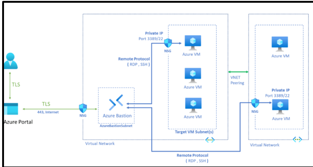
Figure 19 – Azure Bastion Host 21
