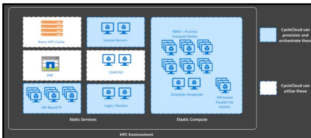
Figure 13 – CycleCloud Deployed Environment 15
